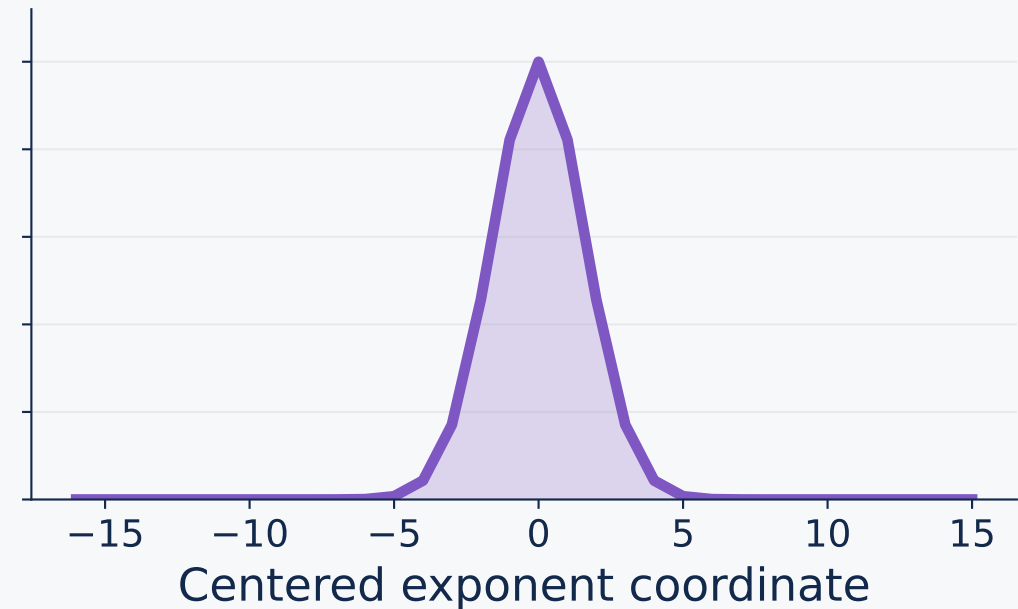
B · finite Gaussian, R=4
